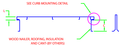
TYPICAL SIDE VIEW
