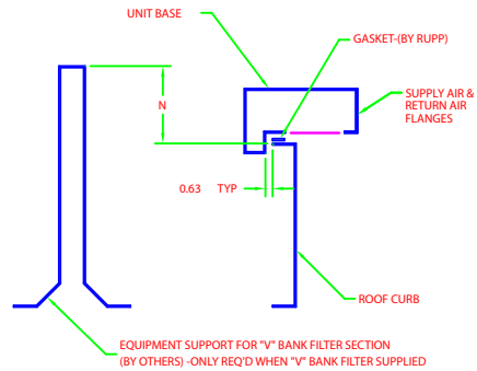
CURB MOUNTING DETAIL
